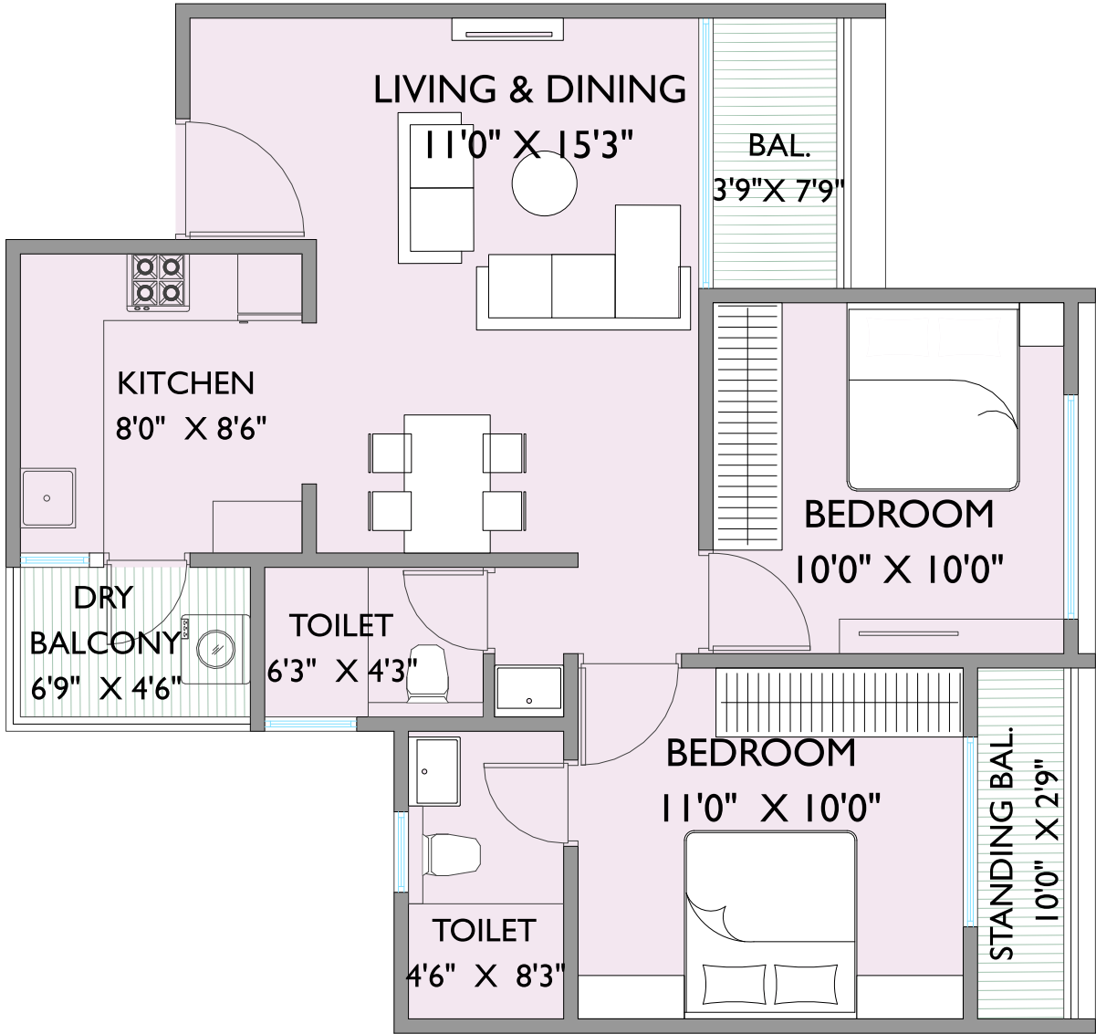
UNIT PLAN - 2 BHK - TYPE D Carpet - 665 Sq.ft.
