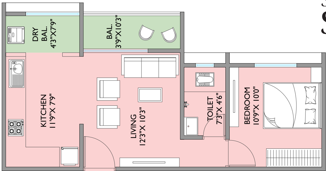
UNIT PLAN - 1 BHK - TYPE B
