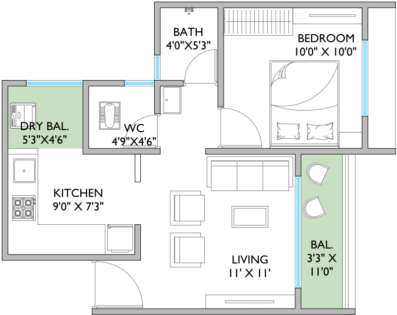
UNIT PLAN - 1 BHK - TYPE C
