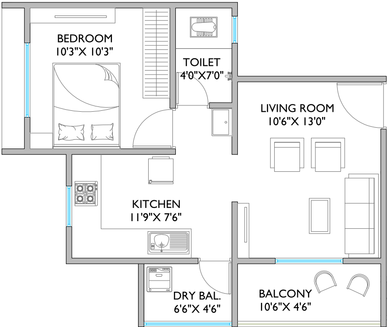
UNIT PLAN - 1 BHK - TYPE E
