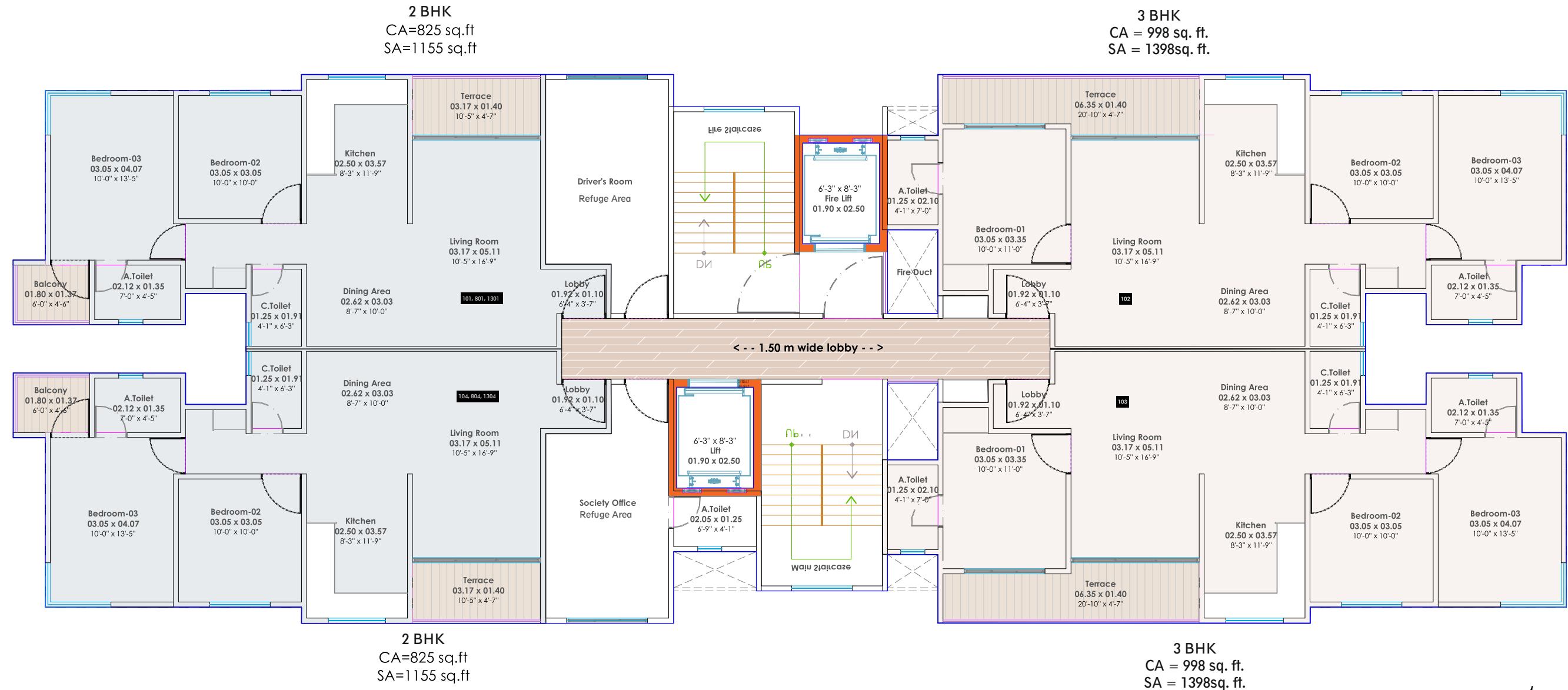
1st, 8th & 13th Floor Plan
