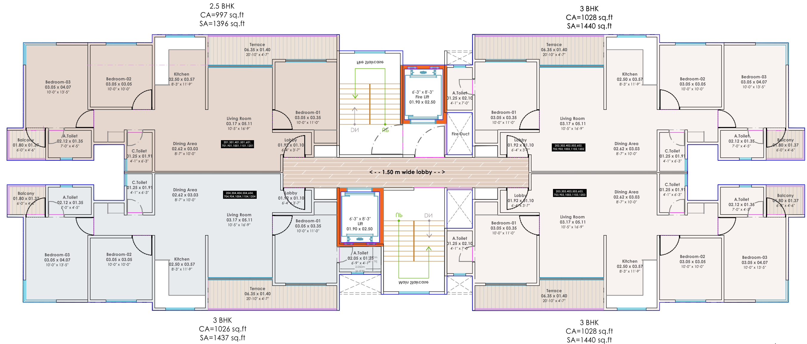
Typical Floor Plan
